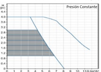
MAGNA3 40-40 F (N) MAGNA3 D 40-40 F
