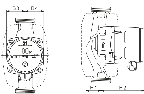
ALPHA1 20-60 150 N (1x230 V)
