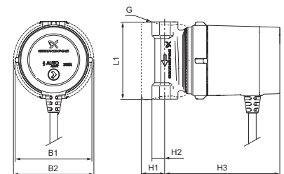
COMFORT 15-14 B(X)A
