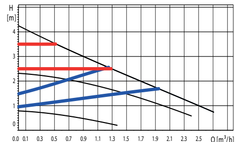
ALPHA1 20-60 150 N (1x230 V)
